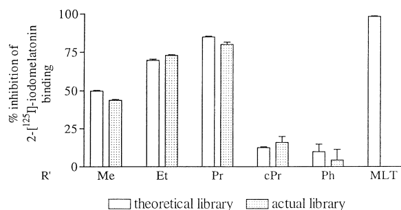
Figure 1. Inhibition of 2\text{-}[^{125}\text{I}] -iodomelatonin binding by compounds 4 ( \text{Ar}=3\text{-MeOC}_6\text{H}_4\text{-} and 2,5\text{-(MeO)}_2\text{C}_6\text{H}_3\text{-} , \text{X}=\text{CH}_2 ) at 5\times 10^{-8}\text{ M} . ( 2\text{-}[^{125}\text{I}] -iodomelatonin was used as the radioligand and the binding assays were carried out using membranes prepared from chicken brain. Membrane aliquots ( 30\text{ }\mu\text{L} ) were incubated in a total volume of 0.25\text{ }\mu\text{L} of Tris-HCl buffer ( 50\text{ nM} , \text{pH } 7.4 ) with 0.05\text{ nM} 2\text{-}[^{125}\text{I}] -iodomelatonin and one concentration ( 10\text{--}7\text{ M} ) of the mixture under test. Each binding assay was performed in triplicate. Non-specific binding was defined with 10\text{ }\mu\text{M} melatonin and represented about 10% of the total binding. Melatonin (MLT) was tested at the same concentration.)
